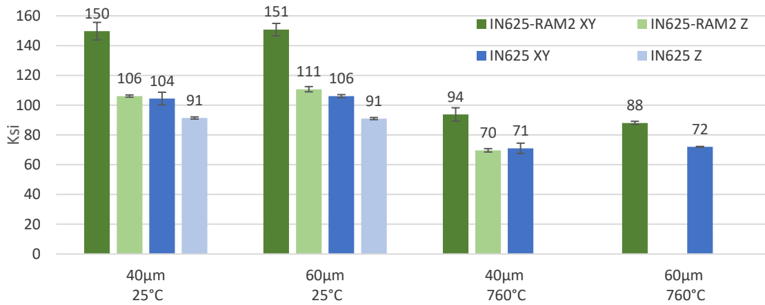
Figure 1: AS-printed IN625-RAM2 yield strength compared to AM IN625 at 25°C and 760°C for 40µm and 60µm print layers printed in the XY and Z direction.
